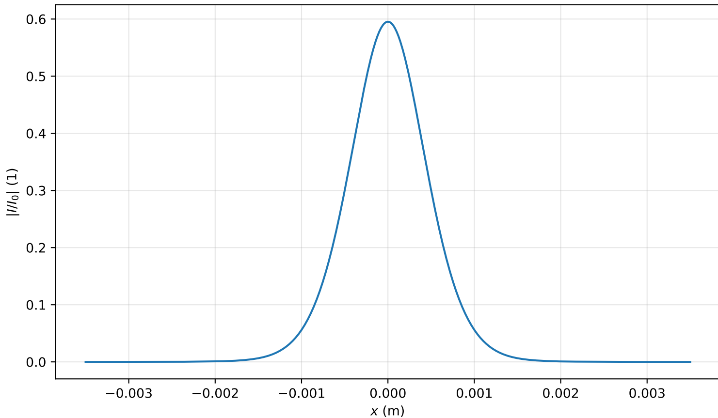
Intensity profile I(x, y = 0, z = 2.866m)/I_0 , P_{in}=0.5P_{cr} , artificial time
